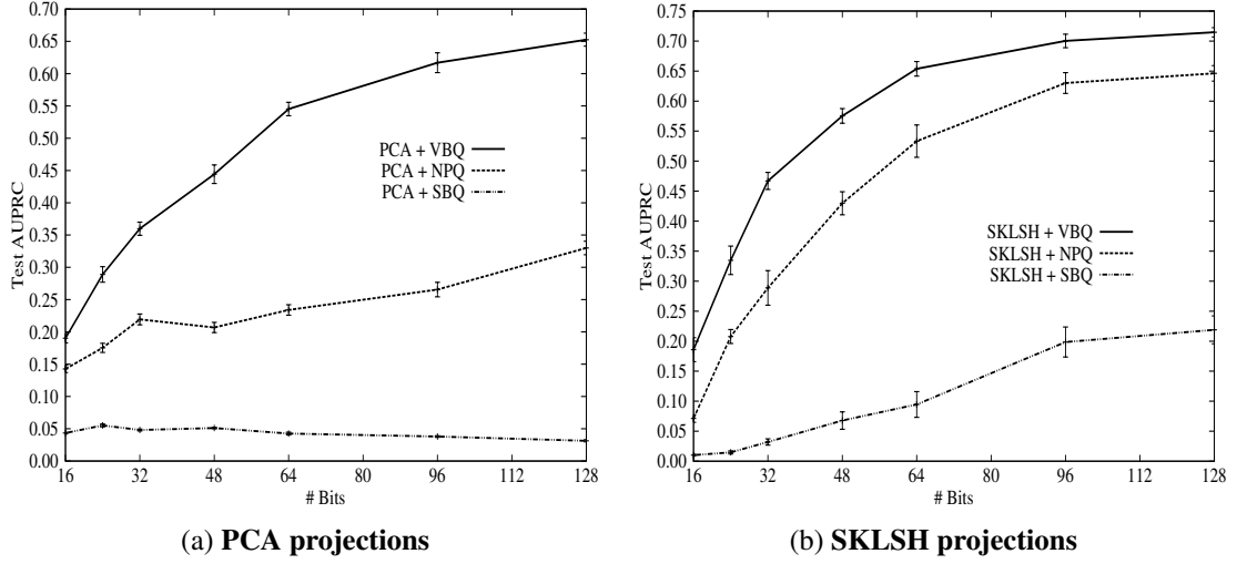
Figure 5.5: AUPRC versus hashcode length on NUSWIDE for PCA (Figure (a)) and SKLSH (Figure (b)) projections. Retrieval results are shown for \text{VBQ}_{\text{bound}} and \text{NPQ}_{\text{opt}} . Bars represent the standard error of the mean.
