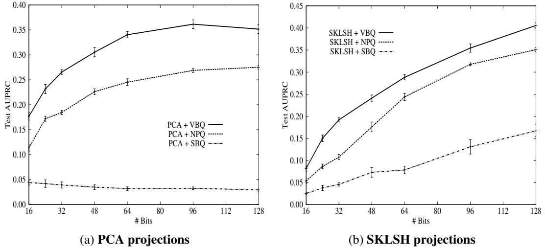
Figure 5.3: AUPRC versus hashcode length on CIFAR-10 for PCA (Figure (a)) and SKLSH (Figure (b)) projections. Retrieval results are shown for \text{VBQ}_{\text{bound}} and \text{NPQ}_{\text{opt}} . Bars represent the standard error of the mean.
