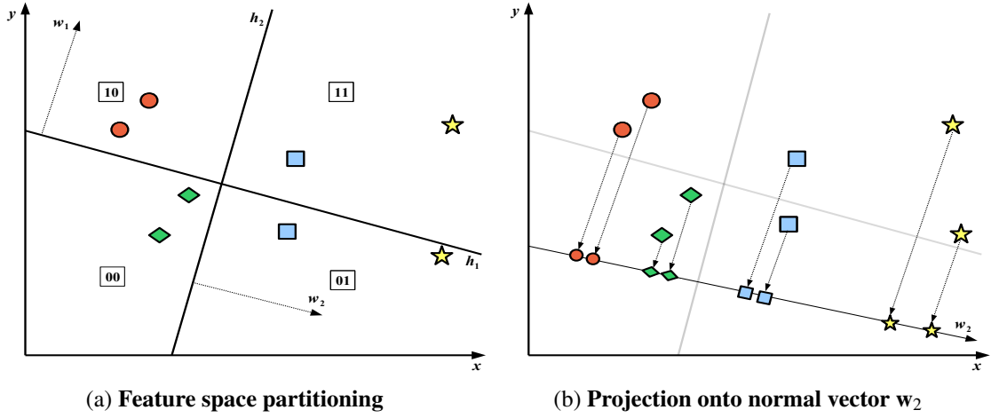
Figure 2.13: Illustration of the projection operation. Methods for projection partition the feature space with a set of hyperplanes. In Figure (a) I show a partitioning of a two dimensional feature space induced by two hyperplanes \mathbf{h}_1 and \mathbf{h}_2 . To determine the bucket index or hashcode of a data-point it is necessary to project the data-points onto the normal vectors ( \mathbf{w}_1 , \mathbf{w}_2 ) followed by binary quantisation. In Figure (b) I show geometrically the result of projection onto normal vector \mathbf{w}_2 . The resulting projections form projected dimension \mathbf{y}^2 \in \mathbb{R}^{N_{trd}} . Section 2.6 examines existing work that seek to position the hyperplanes so that many true nearest neighbours end up close to each other along the resulting projected dimensions.
