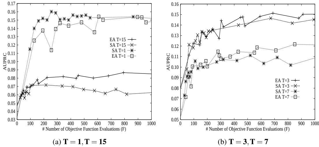
Figure 4.6: CIFAR-10 validation AUPRC for a certain number of objective function evaluations (F) for both simulated annealing (SA) and evolutionary algorithms (EA). Figure (a) shows the result for optimising 1 and 15 thresholds per projected dimension. Figure (b) shows the learning curves for 3 and 7 thresholds.
