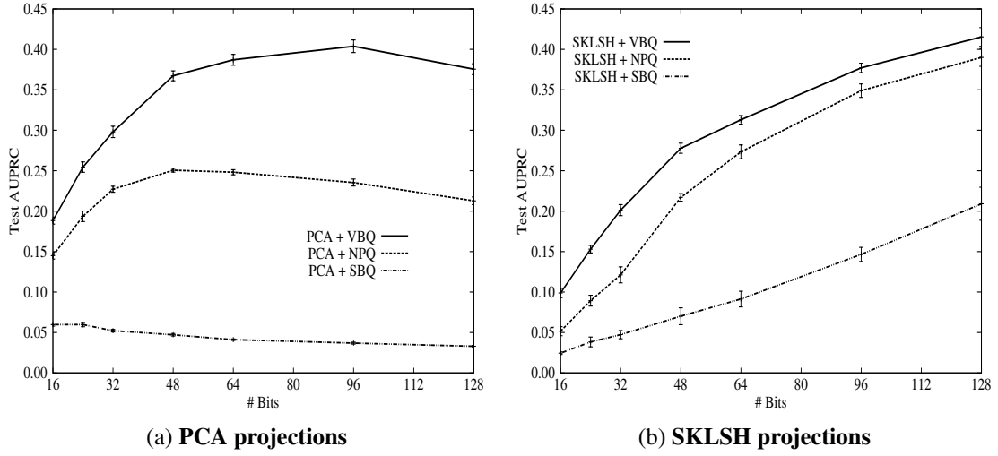
Figure 5.4: AUPRC versus hashcode length on LabelMe for PCA (Figure (a)) and SKLSH (Figure (b)) projections. Retrieval results are shown for \text{VBQ}_{\text{bound}} and \text{NPQ}_{\text{opt}} . Bars represent the standard error of the mean.
