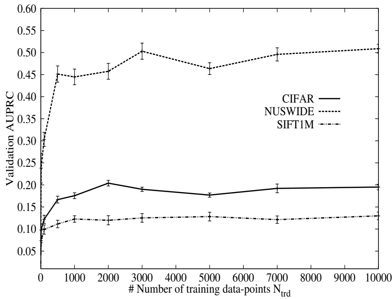
Figure 4.2: The effect of the amount of supervision N_{trd} on the validation dataset retrieval effectiveness (AUPRC). The results are shown for LSH projections with T = 1 threshold per projected dimension (hashcode length of 32 bits). The bars show the standard error of the mean.
