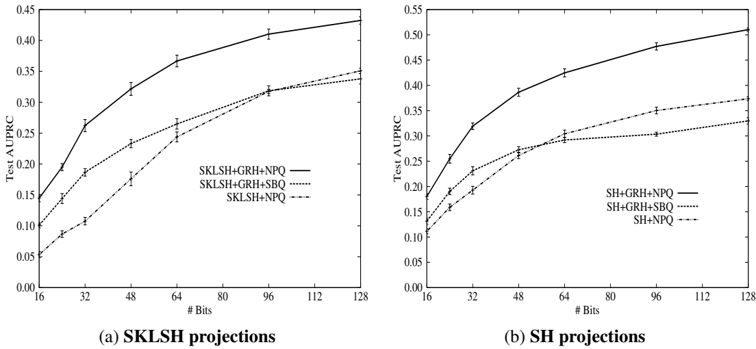
Figure 7.5: Learning the hashing hypersurfaces and quantisation thresholds jointly (GRH+NPQ) versus independently (GRH+SBQ, SBQ) over a hascode length of 16-128 bits. Results are shown for SKLSH projections (Figure (a)) and SH projections (Figure (b)).
