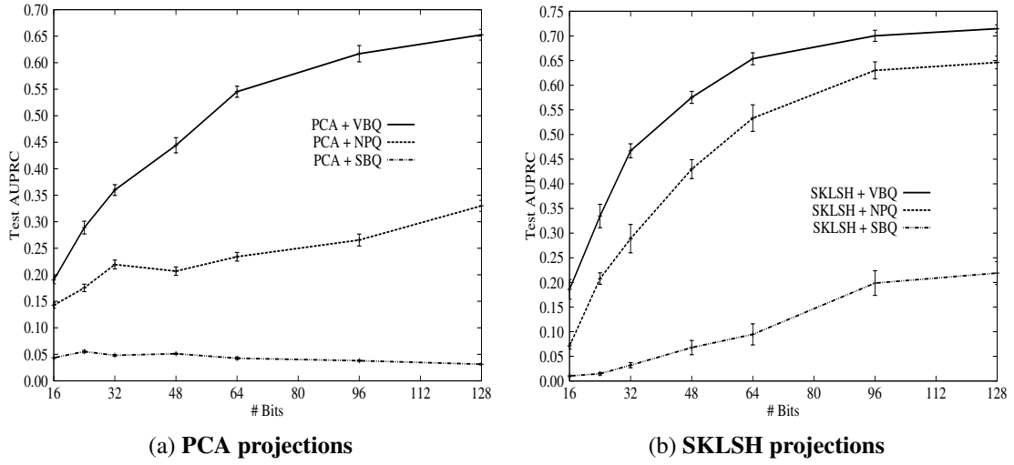
Figure 5.5: AUPRC versus hashcode length on NUSWIDE for PCA (Figure (a)) and SKLSH (Figure (b)) projections. Retrieval results are shown for VBQ_{bound} and NPQ_{opt} . Bars represent the standard error of the mean.
